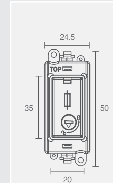
DIMENSIONS (mm)
