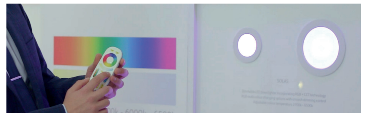
T-CON5 SMART 5 in 1 RF Controller which allows you to wirelessly connect other products to the SMART SYNC system. Suitable for 12V and 24V products.
